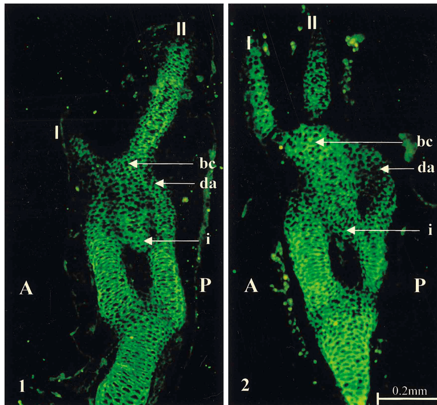
Fig. 7. Skeletal development in the forelimb of two urodeles, the basal hynobiid Salamandrella (1) and the Axolotl (2). In (1), carpus differentiation is proximo-distal with the intermedium (i) in advance of 'bc' and with a relatively early digital arch, da. Apart from early development of digits I and II, this pattern resembles that of other tetrapods (Fig. 8). Immunofluorescence using 3B3 for chondroitin-6-SO4. See Hinchliffe and Vorobyeva, 1999.
