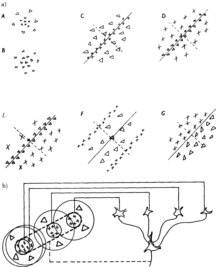
Figure 3. a) Common arrangement of lateral geniculate (A and B) and simple cortical (C–G) receptive fields. X, areas giving excitatory responses ('on' responses); Δ, areas giving inhibitory responses ('off' responses). Receptive-field orientations are shown by continuous lines through field centers; in the figure these are all oblique, but each arrangement occurs in all orientations (Fig. 2 (12)).
